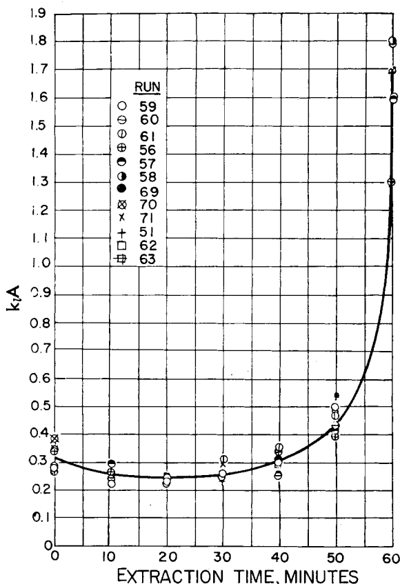
Fig. 4. Correlation of k_t A in continuous countercurrent diffuser.
